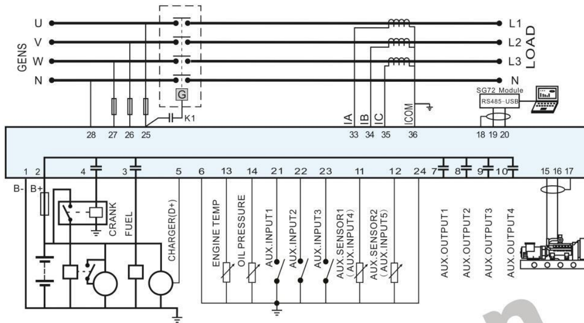
HGM4010CAN Typical Application
